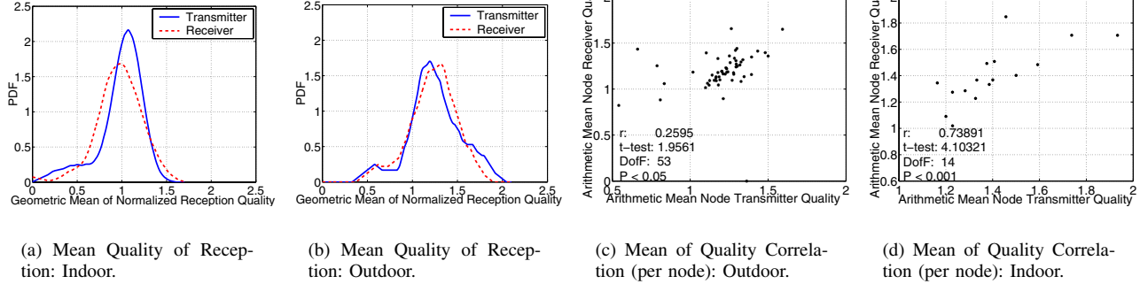
Fig. 9. PDF for Normalized Transmitter and Receiver Quality and Correlation
