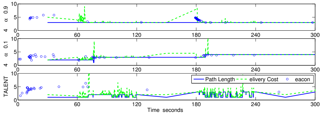
Fig. 16. The path length and the delivery cost of 4B (stable and reactive) and TALENT during a 5 minutes experiment.
