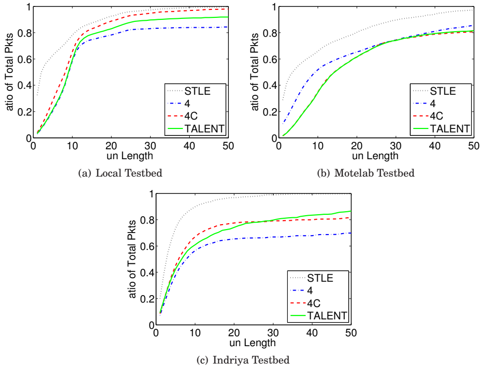
Fig. 18. CDF of the ratio of the packets sent through a particular run length with respect to the total number of packets sent in the data forwarding path. The run length is labeled in the x-axis and limited to [1, 50] range. The results from different link estimators are marked with different line styles.
