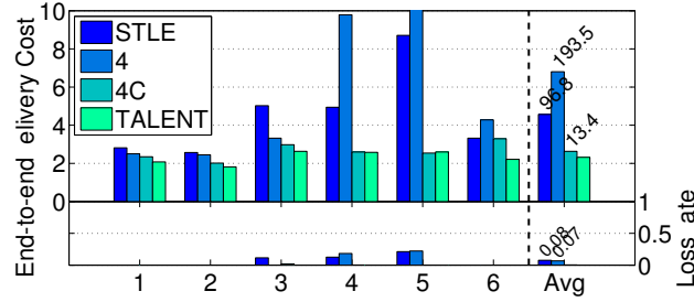
Fig. 19. End-to-end delivery cost and loss rate of local testbed. The experimental settings are described in Fig. 13. Each bar represents the average results of 3 experiments with the same network settings.
