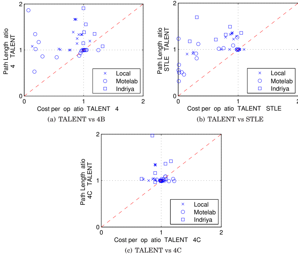
Fig. 17. The average delivery cost per hop ratio of TALENT and (4B/STLE/4C) versus the path length ratio (4B/STLE/4C) and TALENT in all the single sender experiments. The marks above the line x-y = 0 indicate better overall costs of TALENT over the other link estimators.
