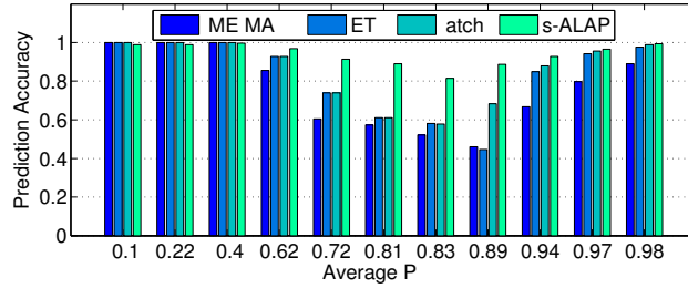
Fig. 24. Prediction accuracy of WMEWMA, ETX, batched trained LR model and LR model with s-ALAP applied to Rutgers dataset. Only 11 out of 112 total links are shown here to represent links with diverse qualities.
