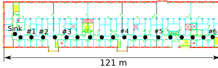
Fig. 13. Local testbed with 57 Tmote Sky motes placed along an corridor of a typical office building. The motes are divided into 19 groups denoted by the black dots. The distance between each node group ranges from 6 to 7 meters, except for the node group in the far left which sits around a corner at the end the corridor. The root node is denoted as Sink and the sender node in each experiment are denoted as #1 to #6. The number of nodes included in each experiment is 5, 6, 11, 25, 42, and 57 respectively.
