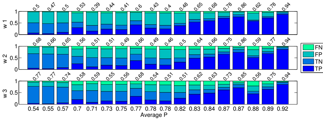
Fig. 5. Prediction accuracy of STLE with different window applied to the intermediate links. The labels on the bottom indicate the link PRR, and the detailed results are marked with different color. The labels on the left of each plot represent the window size, i.e., how many consecutive packets are needed before STLE considers a link high quality.
