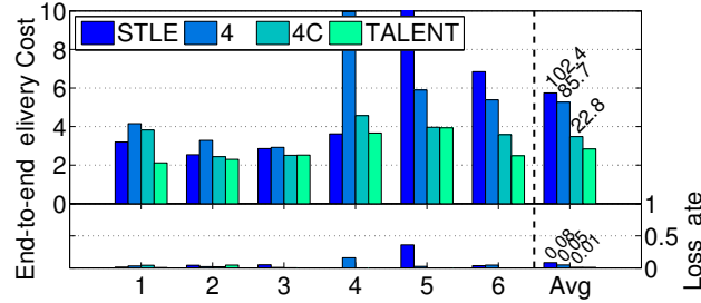
Fig. 22. End-to-end delivery cost and loss rate of variable sending rate and single sender.
