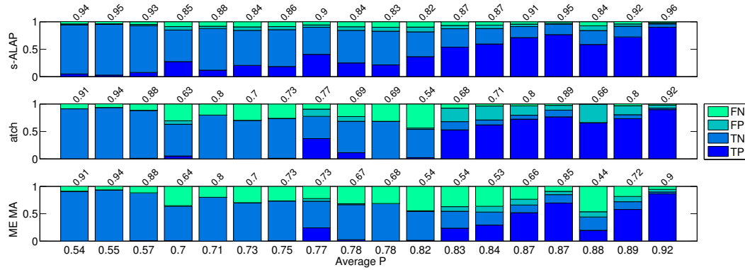
Fig. 3. Prediction accuracy of three prediction methods applied to 19 intermediate links. The numbers on top of each graph shows the prediction accuracy, and the labels on the bottom indicate the link PRR. The detailed results (TP, TN, FP, FN) are marked with different colors for each link.
