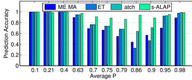
Fig. 25. Prediction accuracy of WMEWMA, ETX, batched trained LR model and LR model with s-ALAP applied to University of Colorado at Boulder dataset. Only 11 out of 130 total links are shown here to represent links with diverse qualities.
